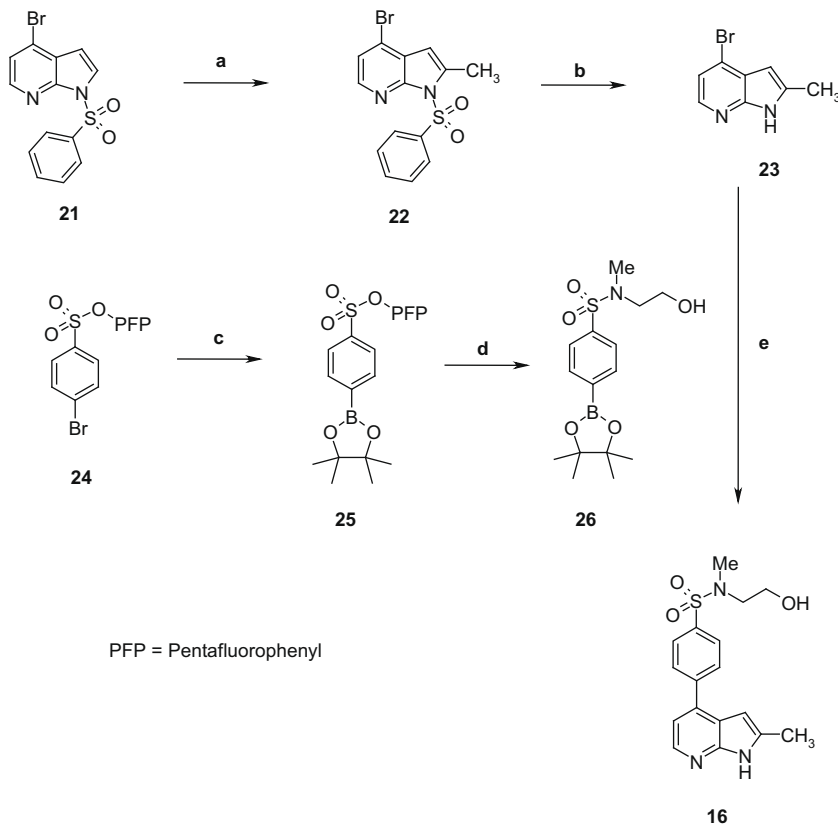
Scheme 1. Reagents and conditions: (a) LDA, THF, -35^\circ\text{C} 30 min then MeI, 2 h, 80%; (b) TBAF, THF, microwave 60^\circ\text{C} , 1 h, 89%; (c) pinacol diboron, PdCl 2 (dppf), dppf, NaOAc, 1,4-dioxane 105^\circ\text{C} , 16 h, 17%; (d) amine, Et 3 N, DMF, microwave 120^\circ\text{C} , 10 min, not isolated; (e) K 3 PO 4 , 2'-(dimethylamino)-biphenyl-palladium(II) chloride dinorbornylphosphine complex, 1,4-dioxane, water, microwave 130^\circ\text{C} , 30 min, 56% for steps d and e.
